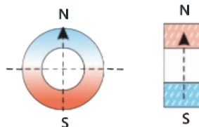
径向充磁 Radial magnetizing
